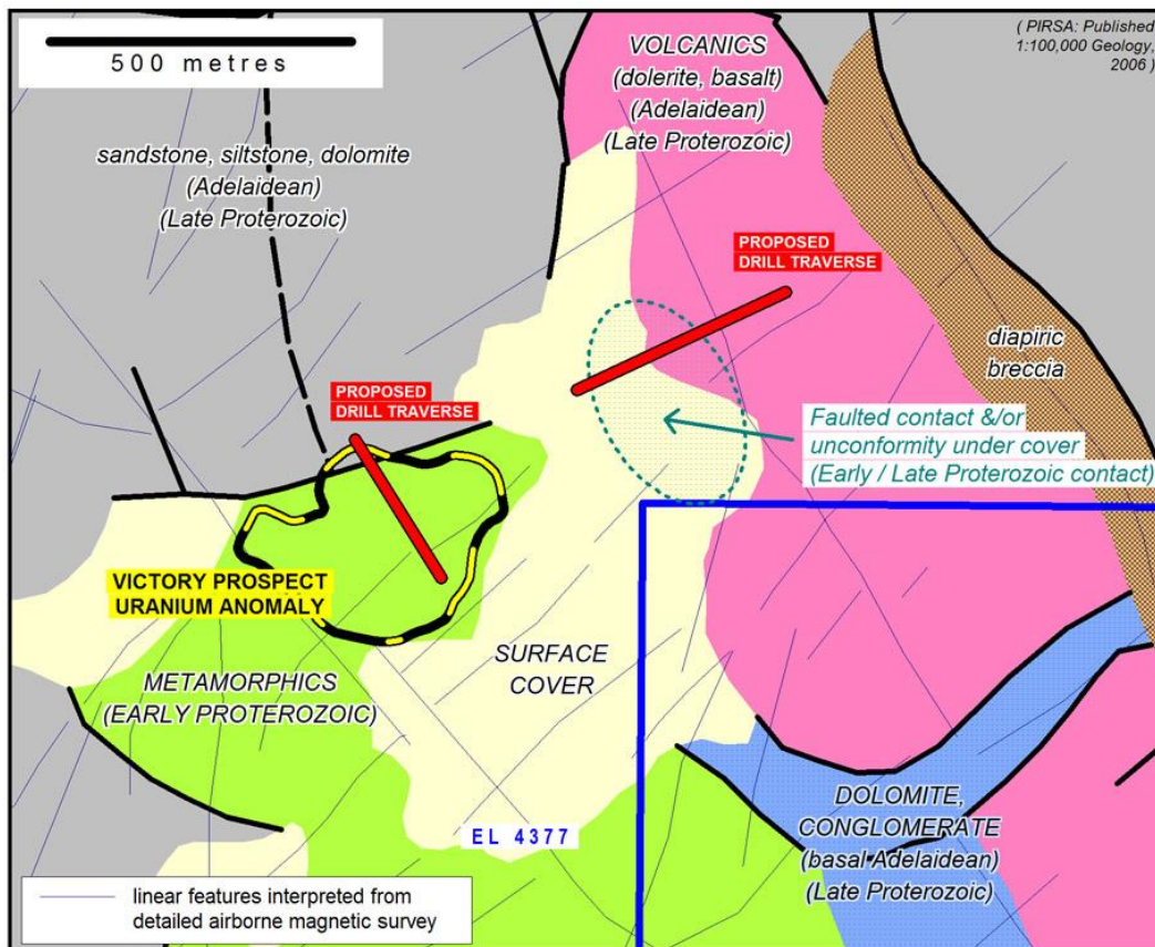
Proposed drill traverses at the Victory uranium prospect, Edward Creek project, South Australia (subject to funding).
