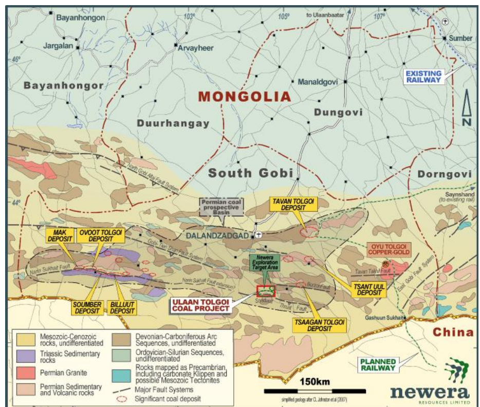
Figure 1: Ulaan Tolgoi licence area within South Gobi regional geology map – showing interpreted boundary of the late Permian coal prospective South Gobi Basin – the Nariin Sukhait and Sönduult thrust faults indicated. Relevant major coal projects indicated.
