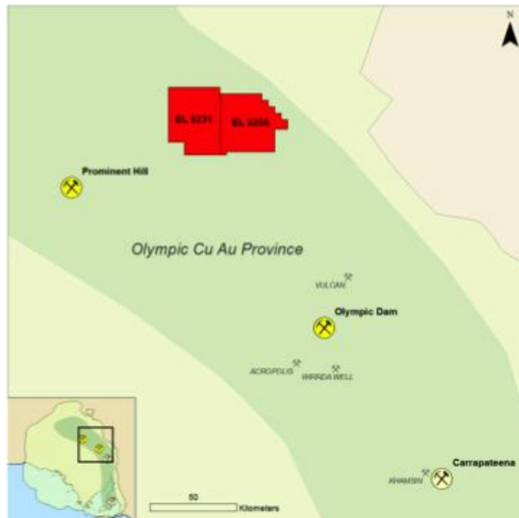
Location Map: GB Energy’s Stuart Shelf Copper-Gold-Uranium project
