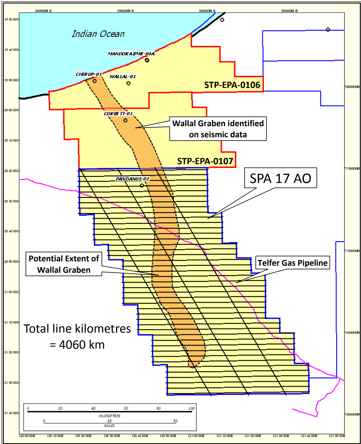
Survey grid of acquired Gravity Gradiometry/Magnetic data in SPA 17 AO
