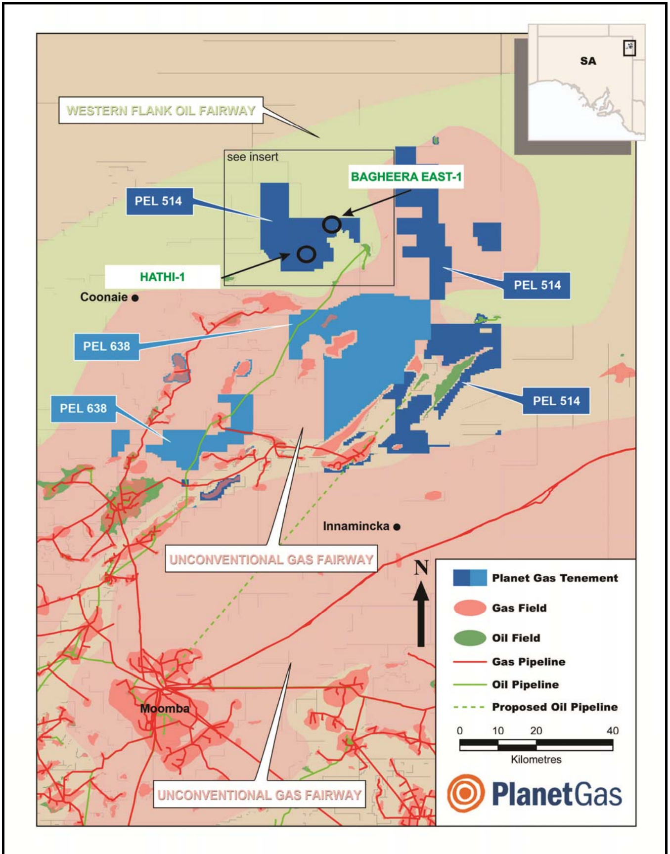
Figure 1: Location of Hathi and Bagheera East Fields
