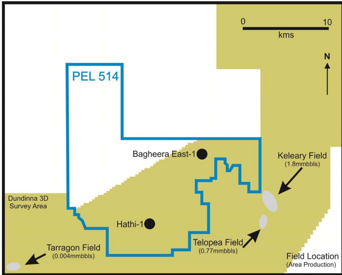
Figure 2: Location of Hathi-1 and Bagheera East-1 Wells
