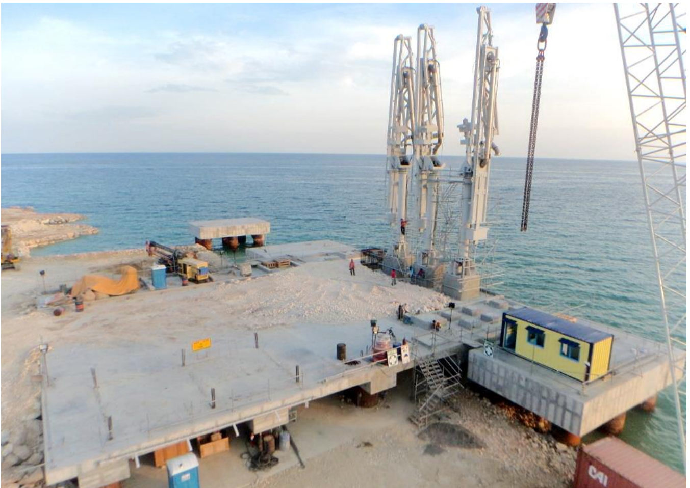
Erection of Marine Loading Arms
