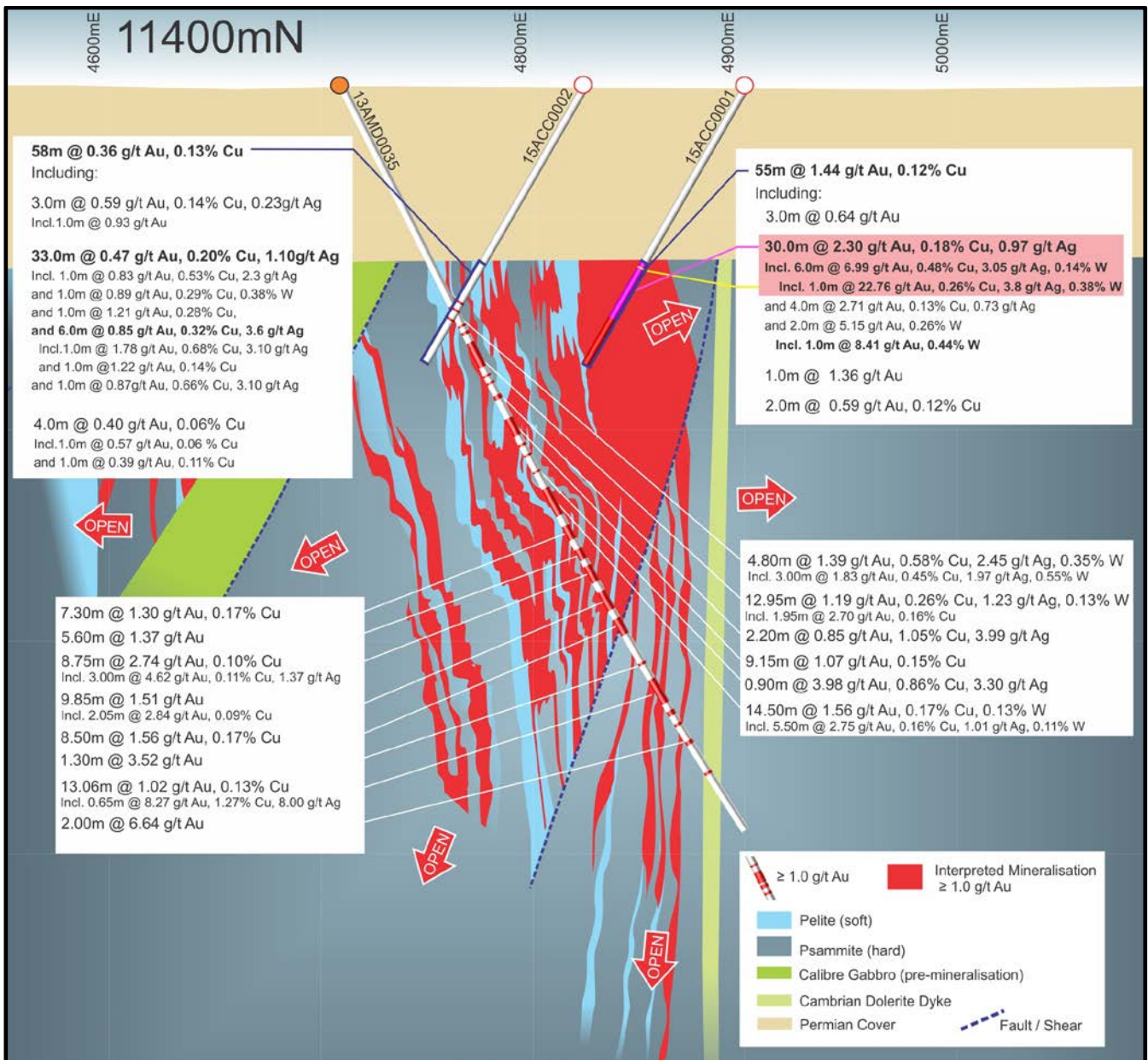
Figure 1: Calibre Deposit 11400 North interpreted (schematic) cross-section showing pre-2015 diamond drillhole 13AMD0035 and 2015 Slim-line RC drillholes 15ACC0001 and 15ACC0002. Interpreted folded interbedded (hard) quartzite and (soft) pelite metasedimentary packages with ≥ 1 g/t gold mineralisation generally internal to or on the margins of the pelite dominated units are also shown (100m grid).
