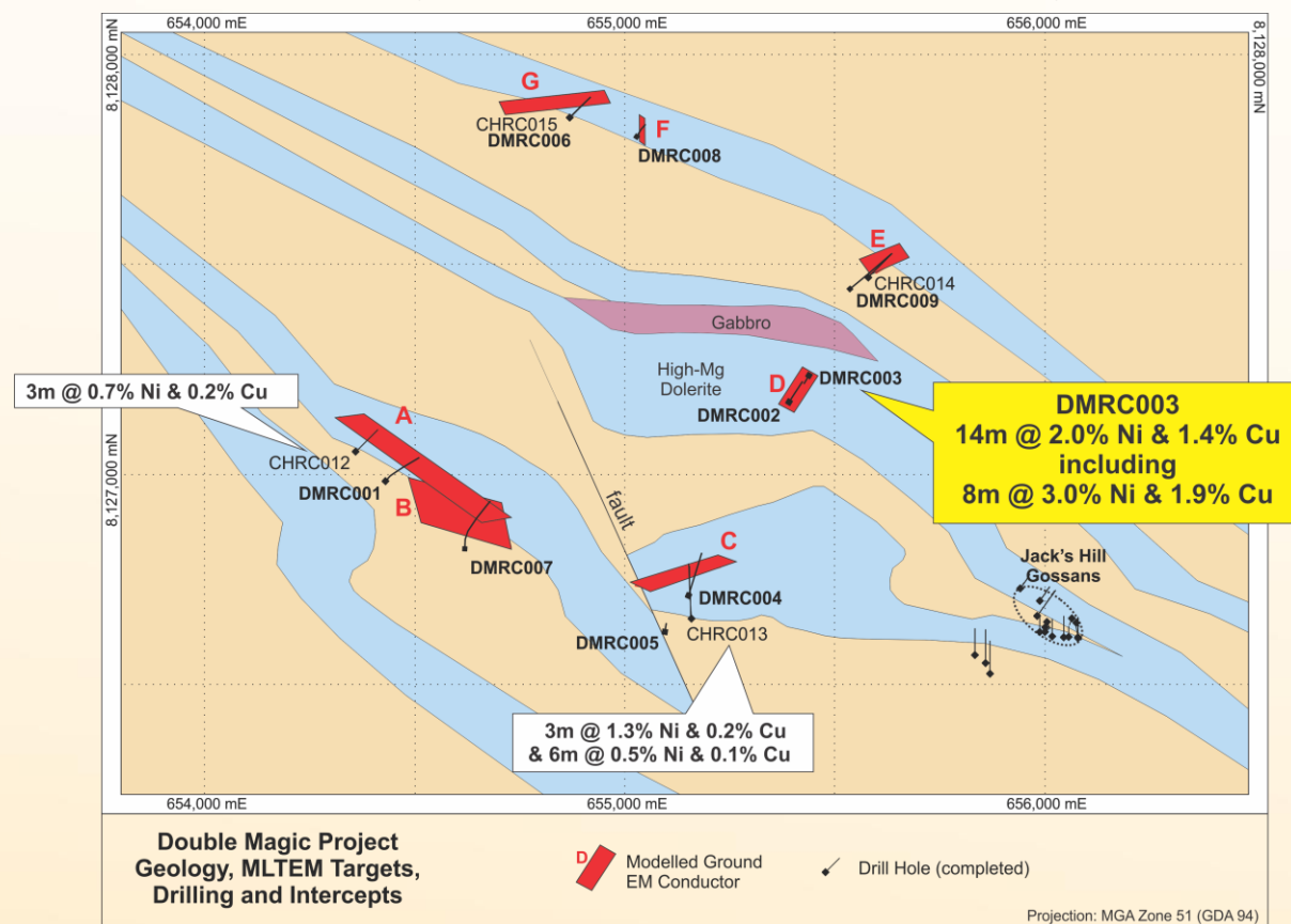
Figure 1. Simplified map of the central area of the Double Magic Project with modelled ground EM conductors, interpreted extent of the Ruins Dolerite/Gabbro, all completed drill hole collars and traces, with selected drilling results.
