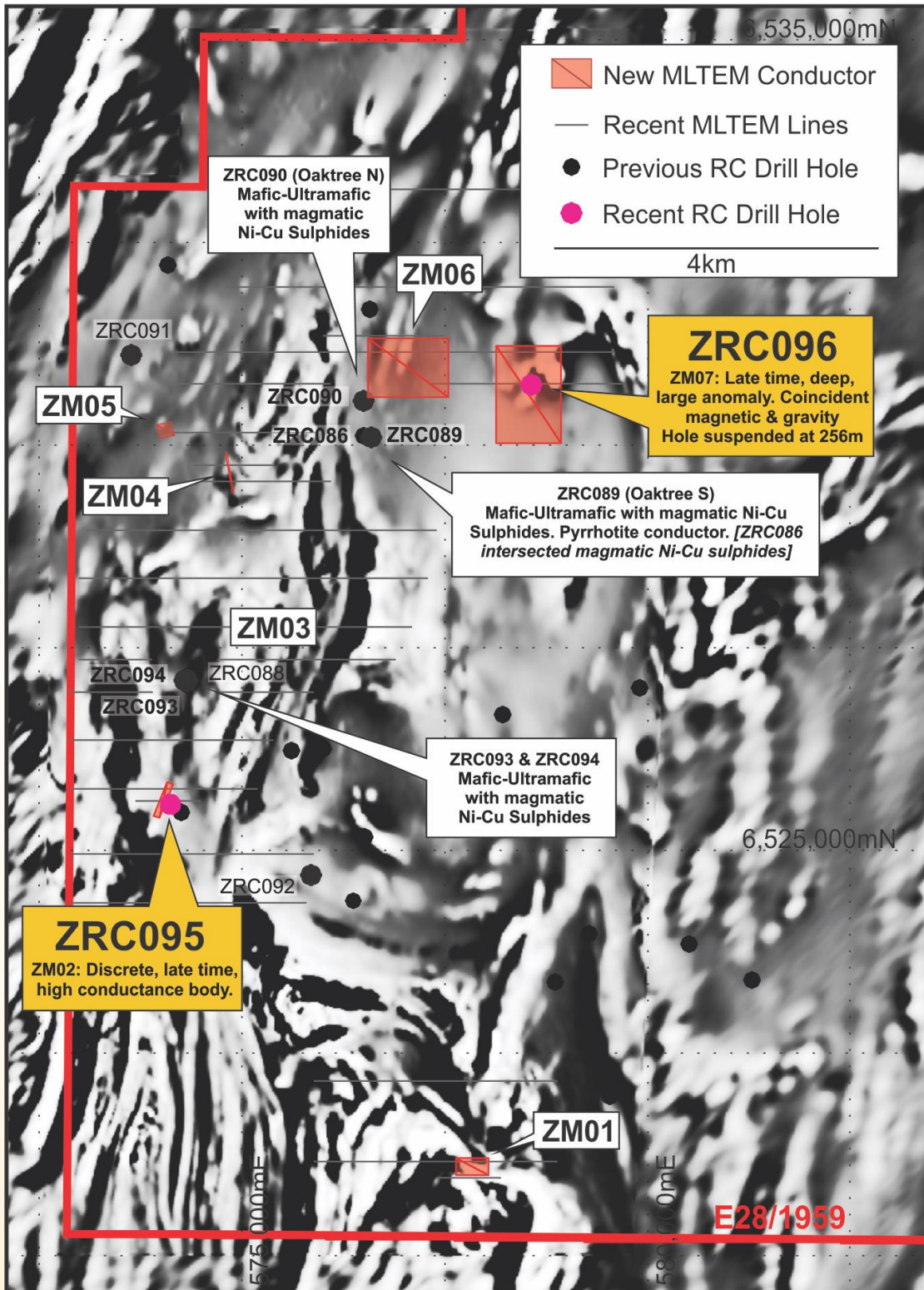
Figure 4. Location of recent drill holes at the Zanthus Project, new MLTEM conductors (e.g., ZM07), recent MLTEM lines, previous drill holes, over airborne magnetics (1VD). Also highlighting drill hole locations with magmatic nickel-copper sulphides.
