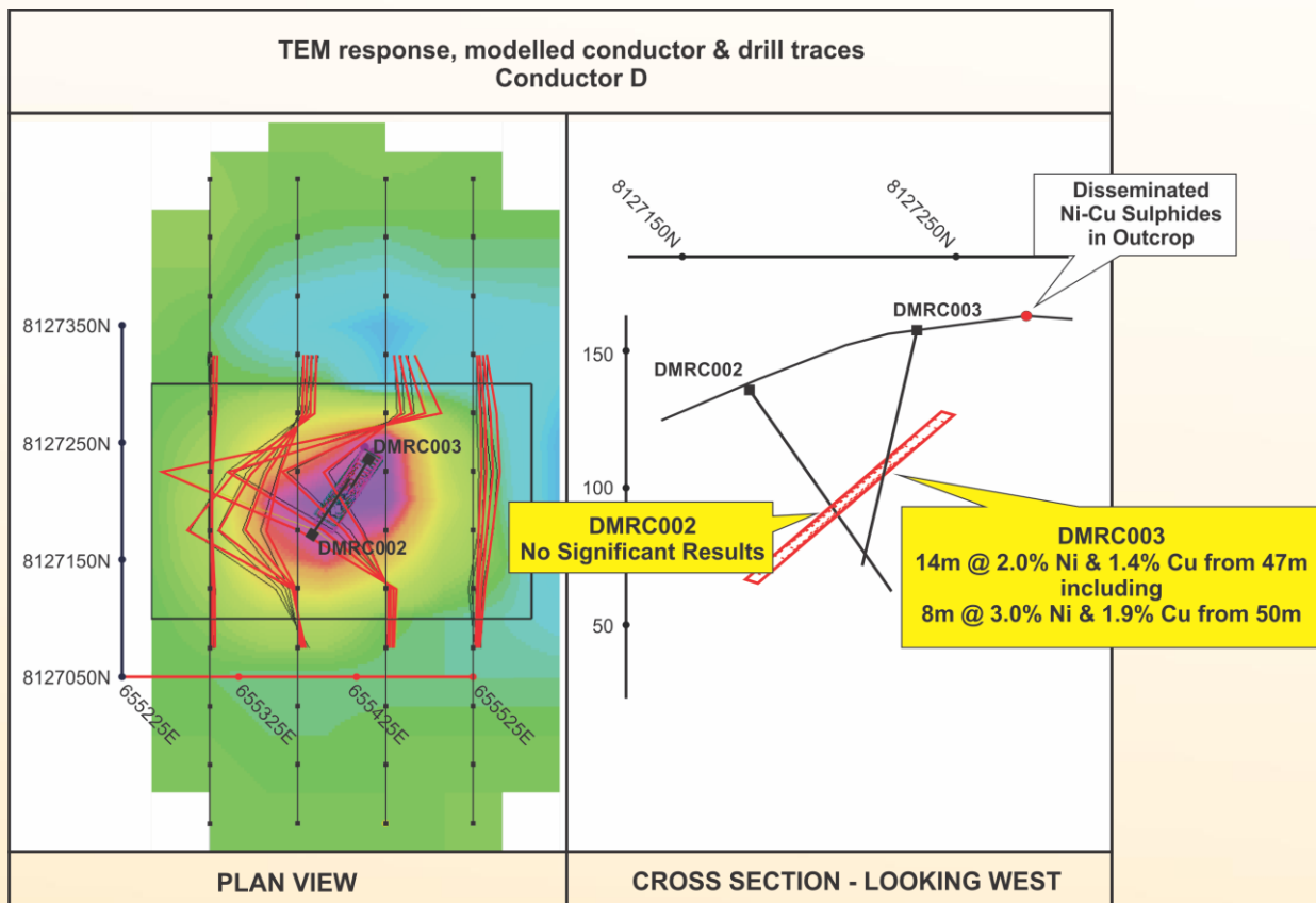
Figure 2. Conductor D, Plan view showing TEM response, stations, modelled EM plate and drill traces, Cross section, showing drill traces, modelled EM plate & intersection.
