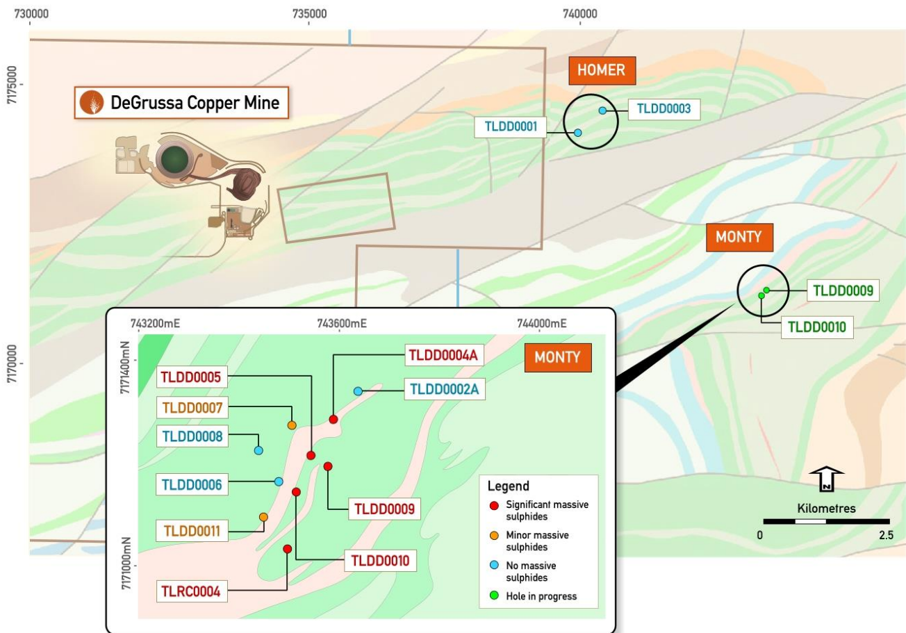
Figure 2 – Plan view showing collar locations of recent exploration drilling at Monty.
