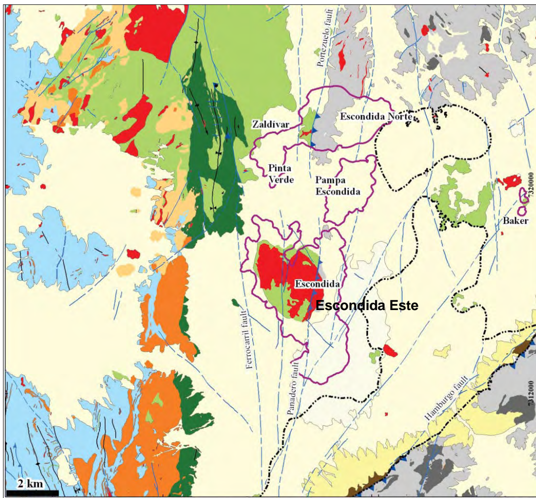
Figure 3: Regional geology setting, after Hervé et al., 2012
