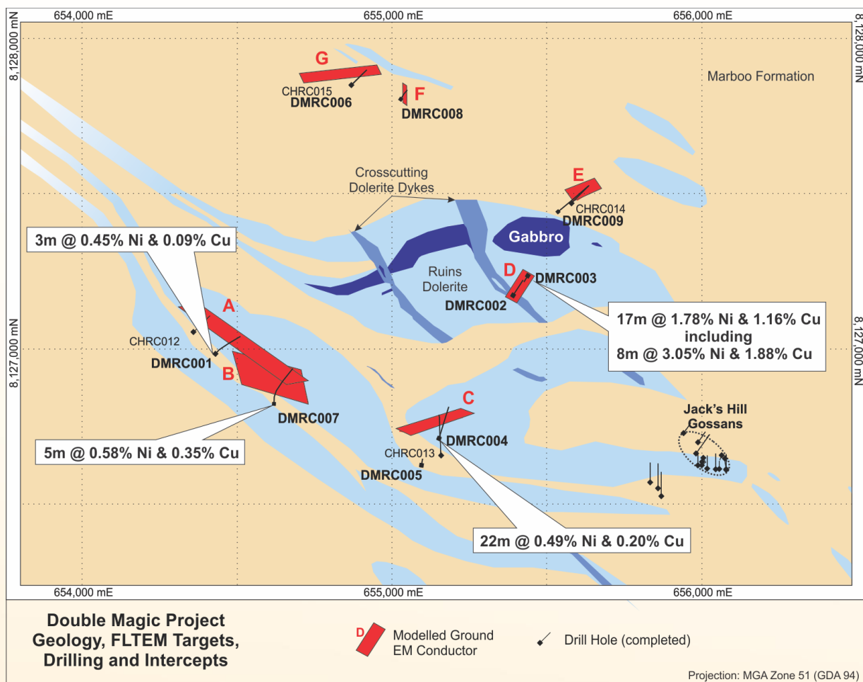
Figure 2 – Simplified map of the central area of the Double Magic Project with modelled ground EM conductors, interpreted geology, all completed drillholes, and selected Buxton drilling results
