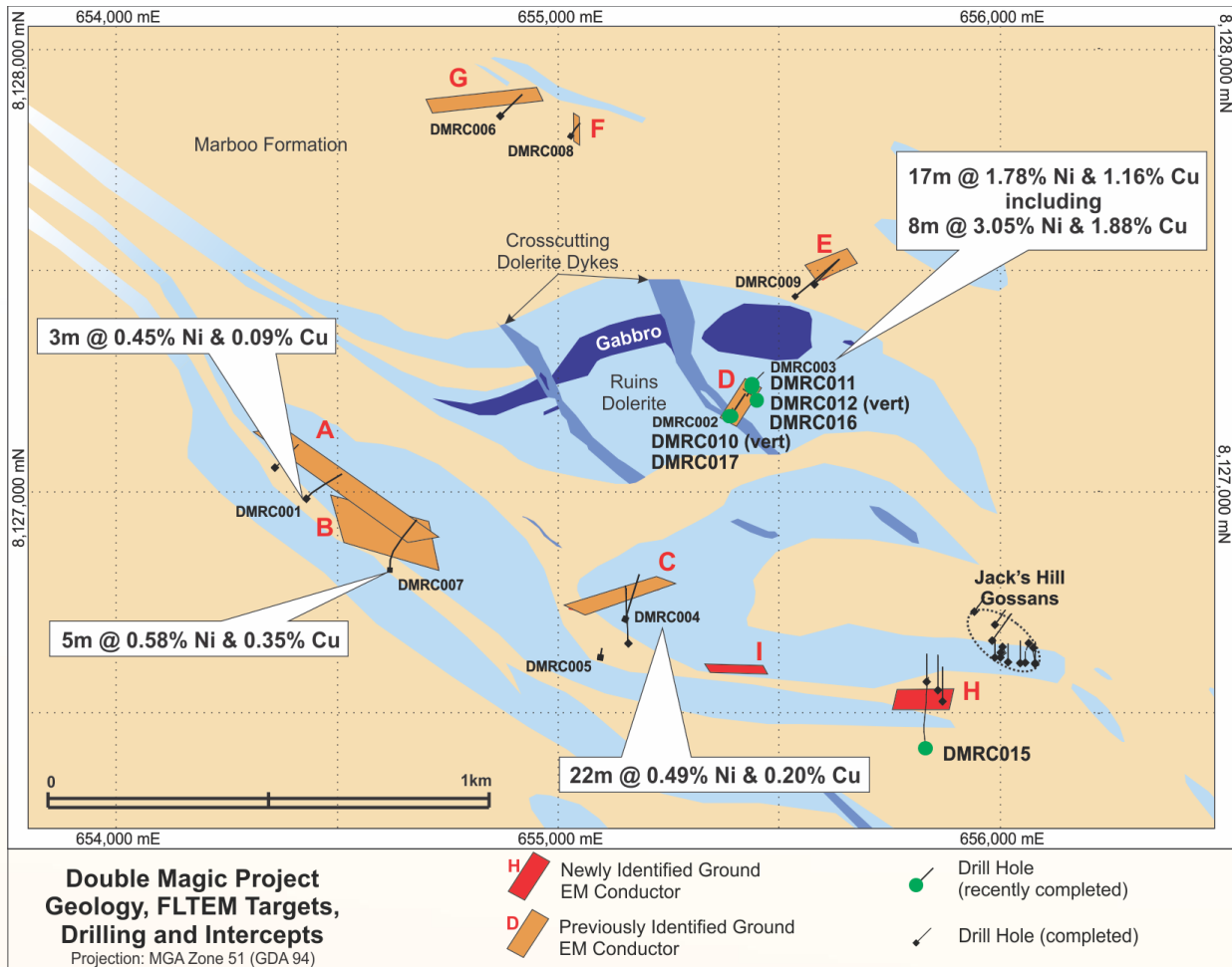
Figure 3 – Simplified map of the central area of the Double Magic Project with modelled ground EM conductors, interpreted geology, all completed drillholes and selected Buxton drilling results
