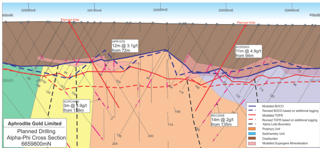
Figure 3- Cross Section 6659800mN showing the depth extend to the transitional zone
