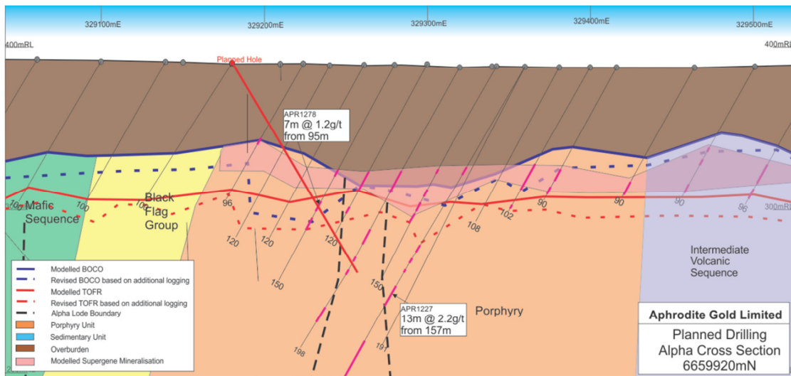
Figure 2- Cross section 6659920mN showing the depth extend to the transitional zone
