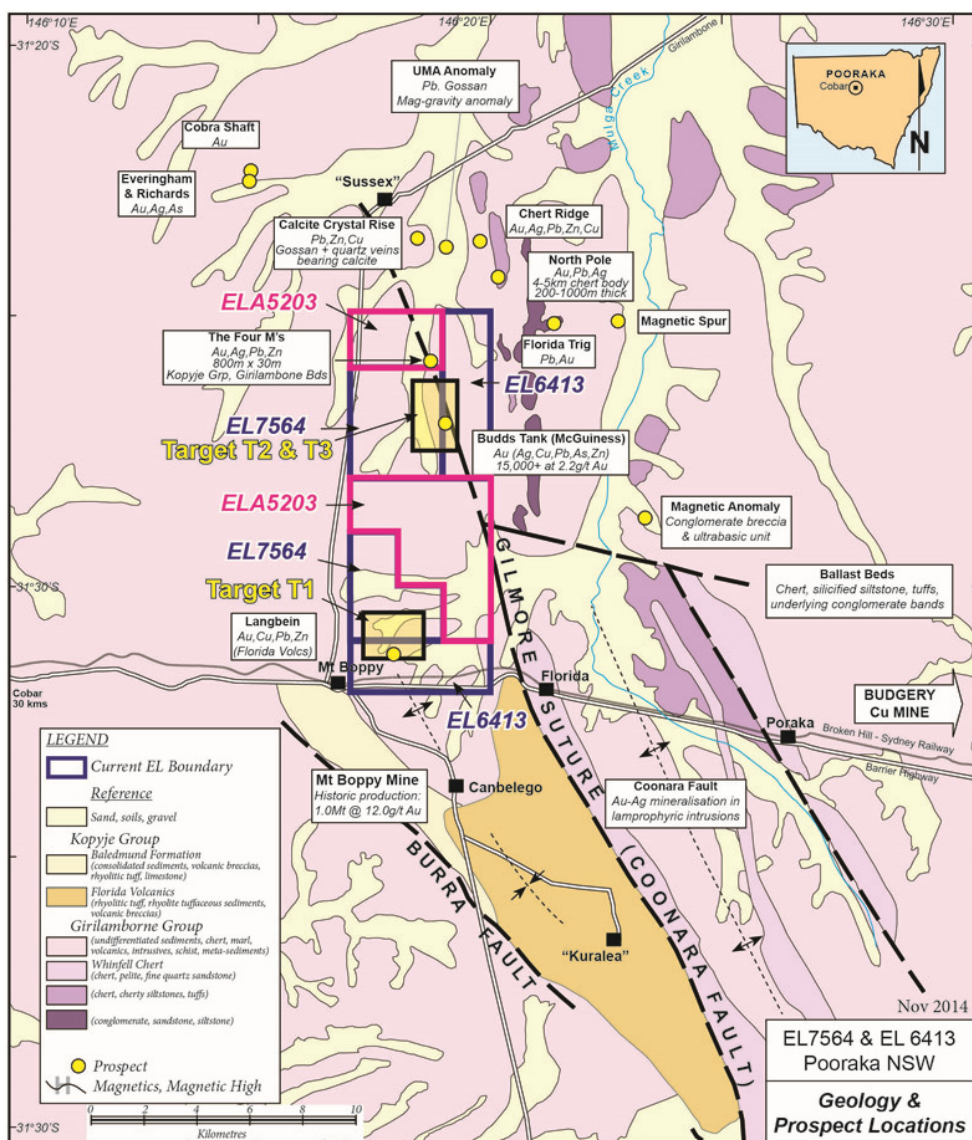
Figure 4 - Geology and Prospect Locations-- Pooraka Project
