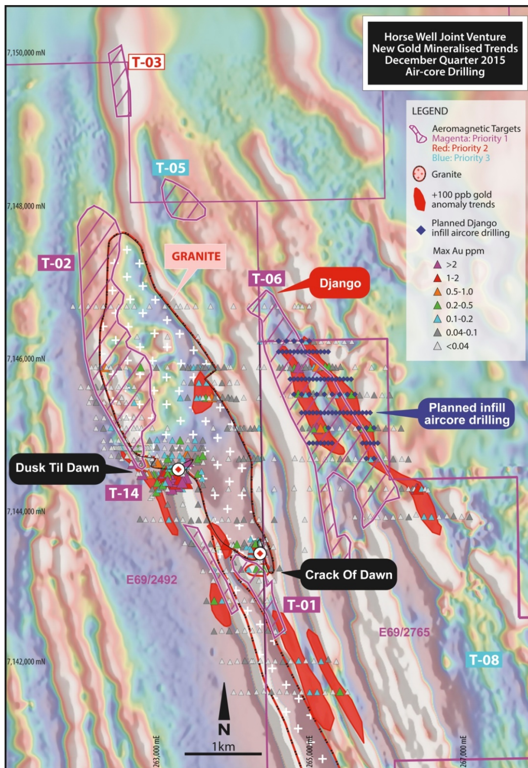
Figure 1 Regional +100ppb Au anomalous trends from December quarter 2015 air-core drilling
