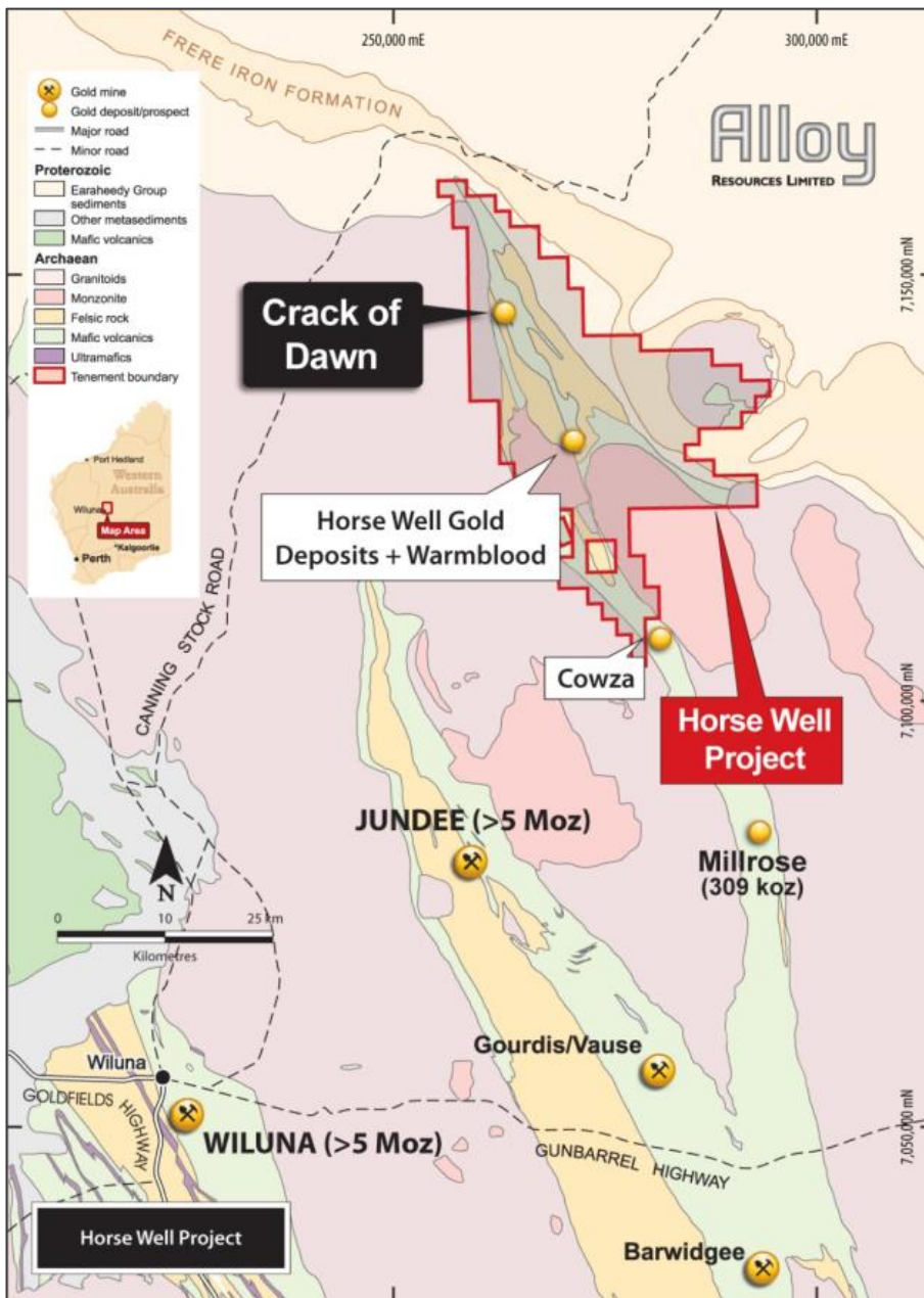
Figure 2 Horse Well location on regional geology
