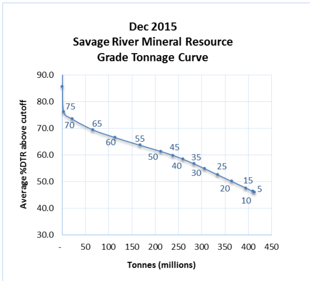
Figure 4 - Grade Tonnage Curve, Savage River
