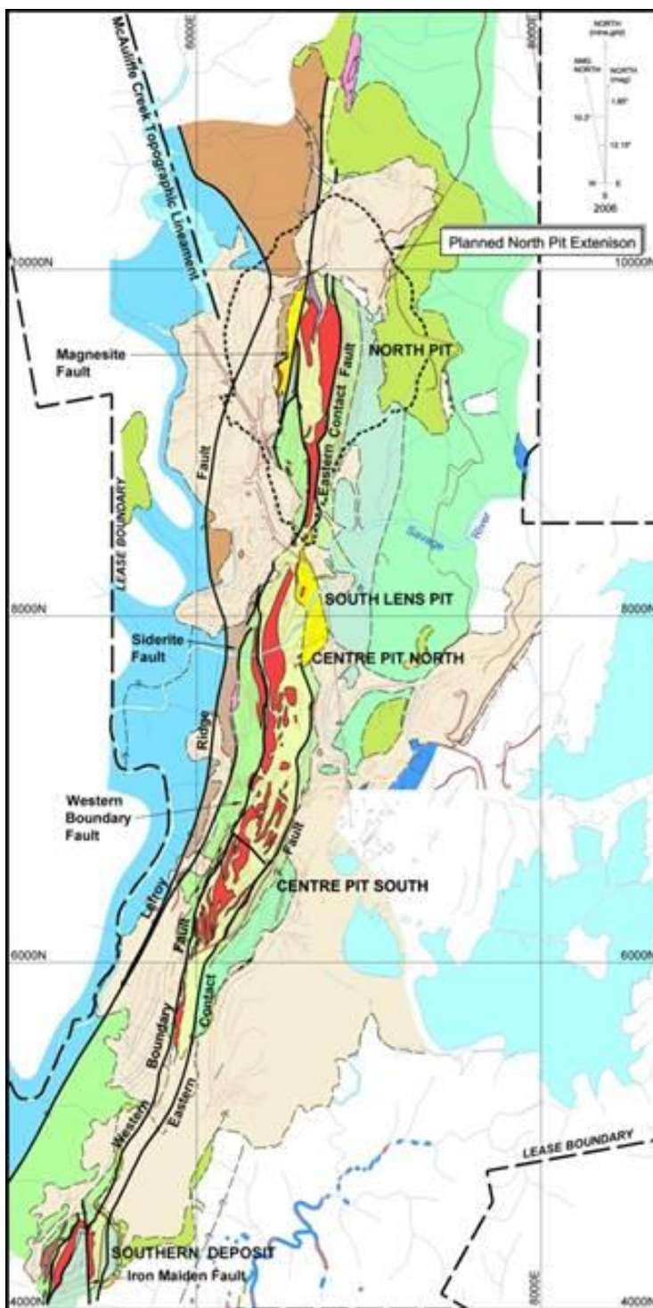
Figure 5 Regional Geology (2008)
