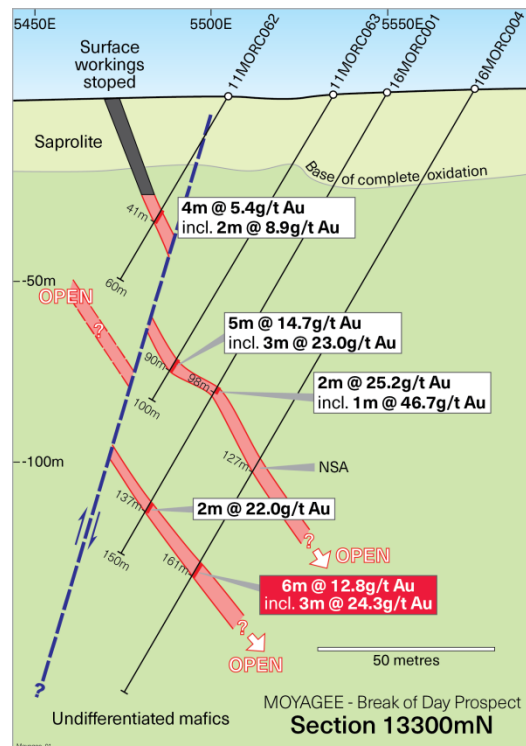
Figure 3: Break of Day cross section showing RC drill holes on section 13300mN (local grid)
