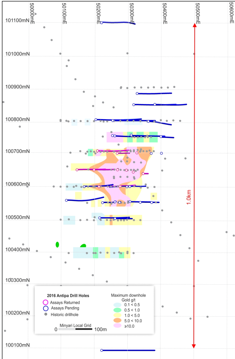
Figure 1: Minyari Deposit plan view showing historic drillhole locations (including significant downhole intersections), 2016 Phase 1 RC drillhole collar locations (including significant downhole intersections) (pink-assays received, blue – assays pending)
