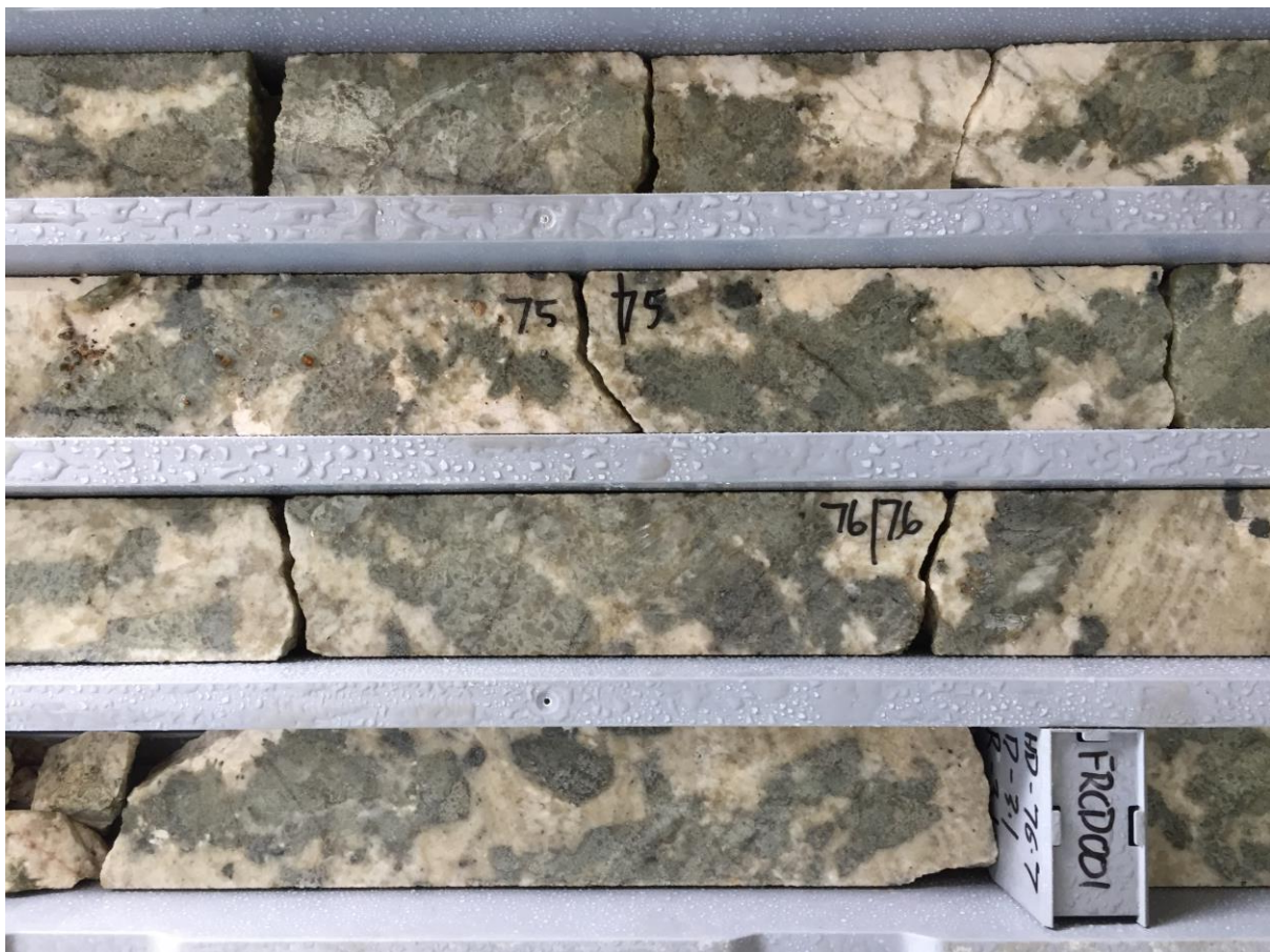
Figure 1. Large green spodumene crystals making up a high proportion of pegmatite volume hosted by lighter coloured (white) feldspar and quartz. 74m – 77m FRDD001 (HQ), Grants Prospect, Finniss Lithium Project NT.
