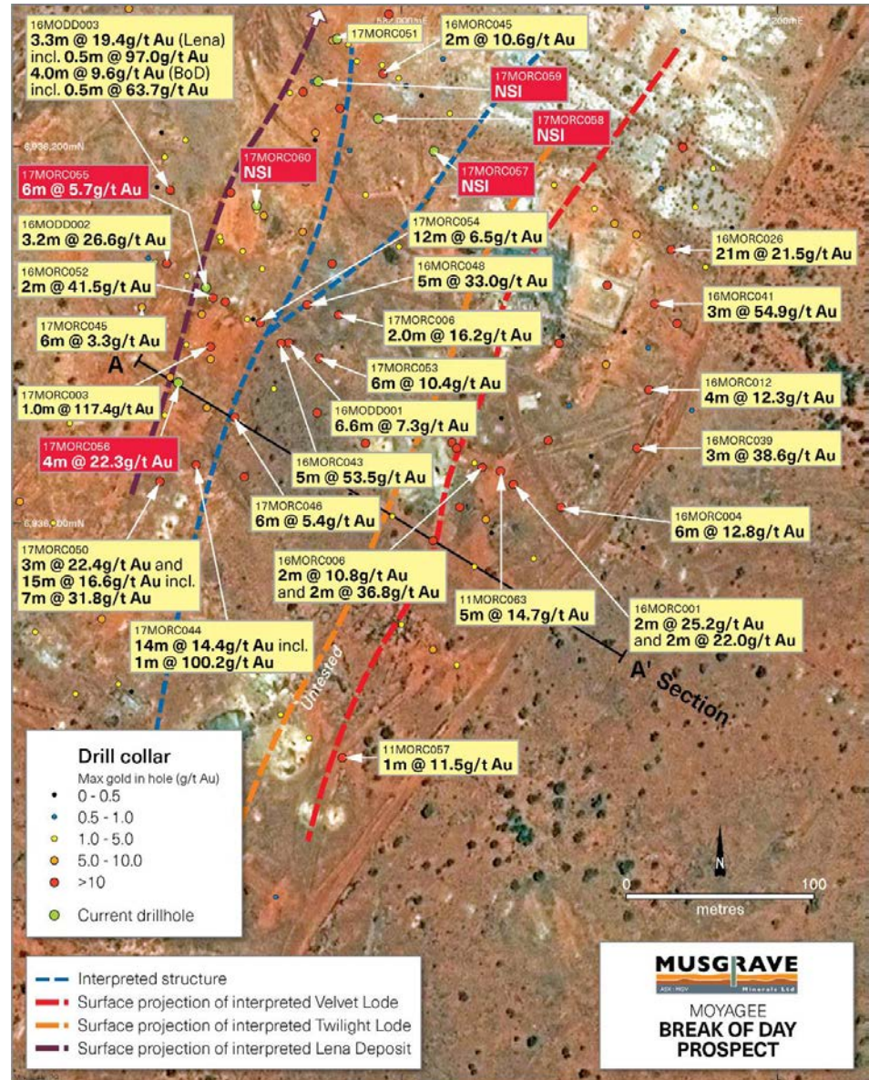
Figure 1: Location plan showing maximum gold in hole plotted at the drill hole collar and significant intersections for the Break of Day gold prospect
