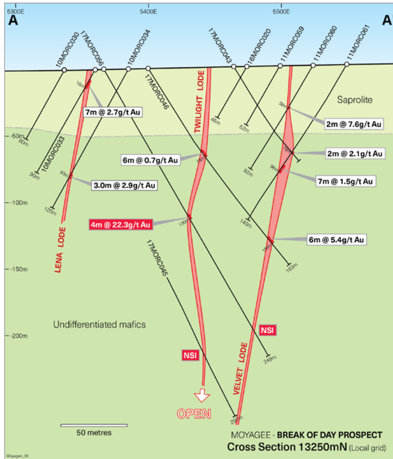
Figure 2: Break of Day cross section 13250mN – local grid (vertical section through mineralisation)
