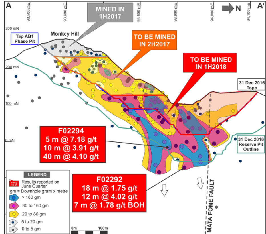
Tap AB1 longsection showing forecast staged pit mining schedule and new drill results
