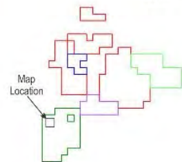
Figure 6. Soil pXRF survey area (Eight Mile), Cu pXRF soil grid results, and rock chip samples thematically mapped by Co content
