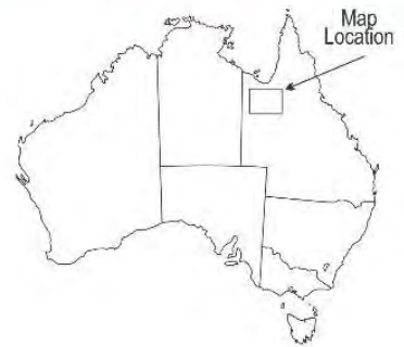
Figure 9. ActivEX Limited Cloncurry Copper and Gold Project regional geology, tenements, mines and prospects
