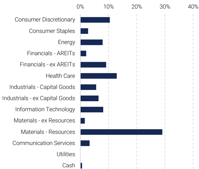
Fig 3. Sector Weights
