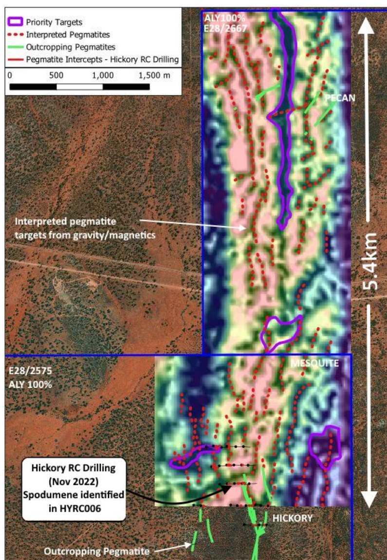
Figure 8: Karonie Project detailed gravity survey area
