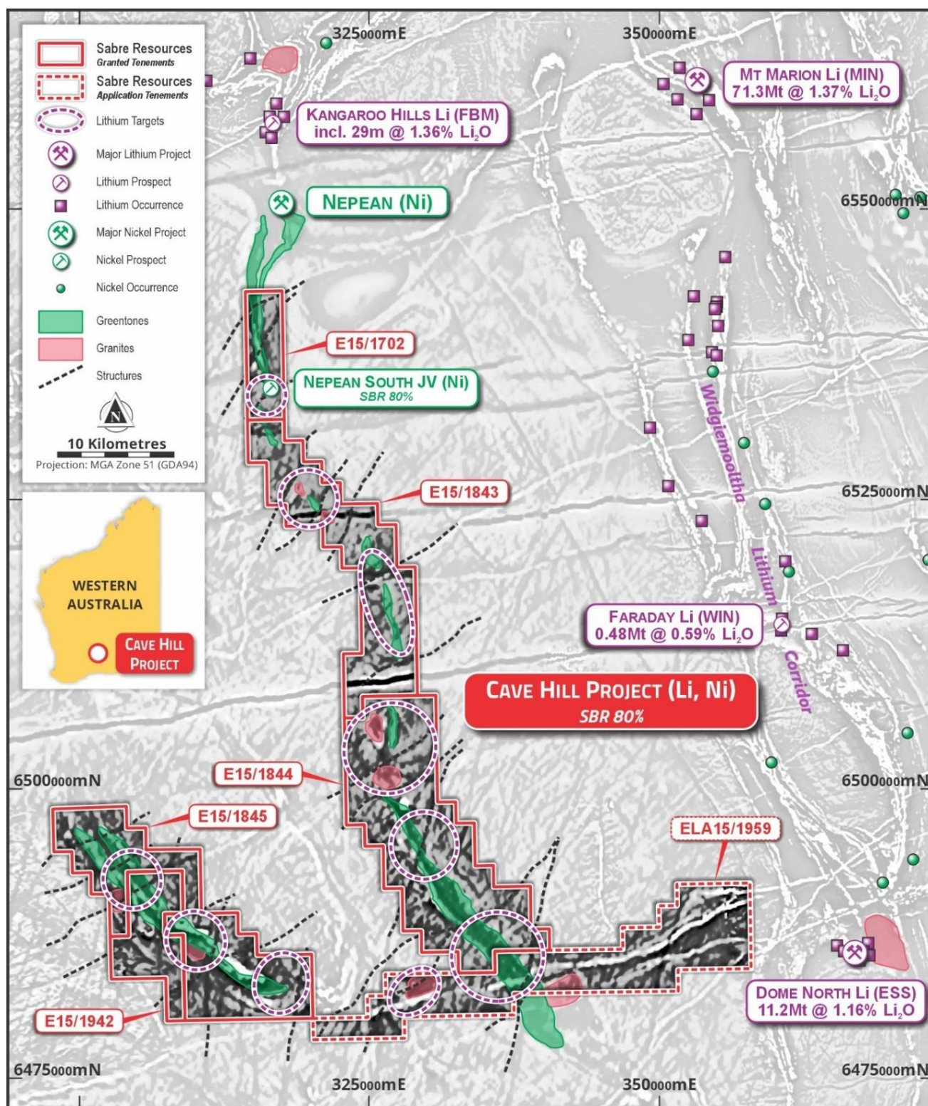
Figure 9: Cave Hill Project tenements on aeromagnetics with other significant lithium projects in the region.
