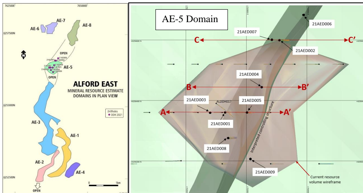
Figure 5: MRE Mineralisation Domains (left); Domain AE-5 showing drillhole collars (right)
