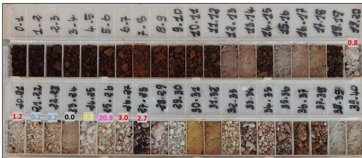
Figure 6: BKRC023 chips showing 9m @ 3.3g/t intercept from 19m.
