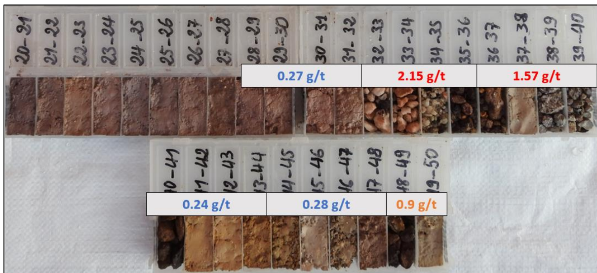
Figure 13: SDAC013 rock chips showing gold grades (g/t)
